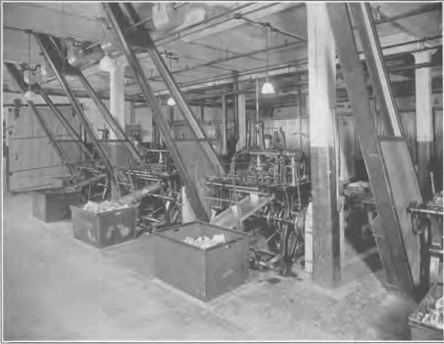
Carton Machines
